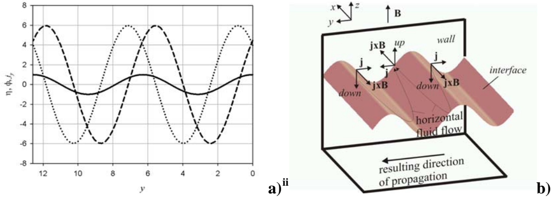
FIG. 6. (a) Functions \eta (solid line), \phi (broken line), and j_v (dotted line) at x = 0 , t = 0 for \beta = 100 , and k_y = 1 and (b) schematic diagram of the mechanism of instability
