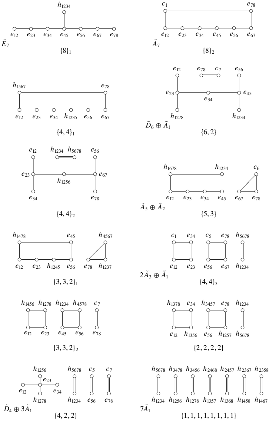
Figure 1 Configurations of vertical divisors on extremal fibrations
