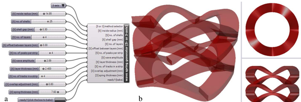
Figure 8 - Use of (a) the developed Grasshopper 3D cluster to generate (b) a closed mesh ready for G-code generation
