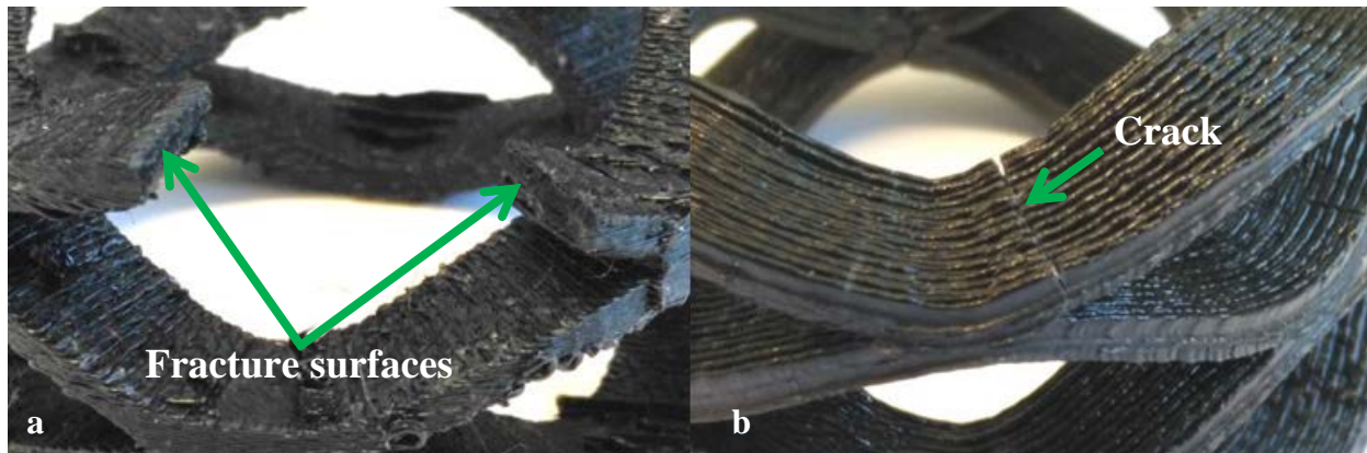
Figure 13 - A comparison of wave springs produced via (a) 3-axis and (b) 5-axis ME
