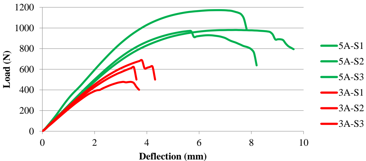
Figure 12 - A graph of force profiles generated using compression testing data
