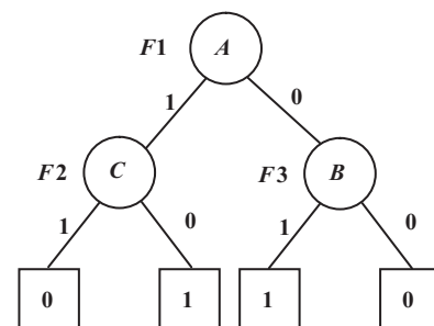
Fig. 3 SFBDD for the fault tree in Fig. 2
