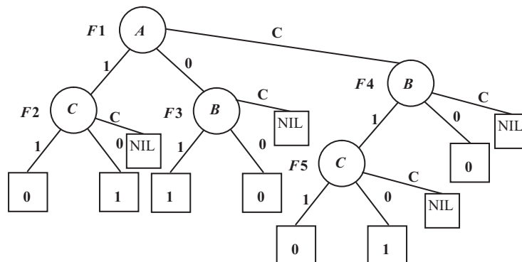
Fig. 5 TDD for the fault tree shown in Fig. 2
