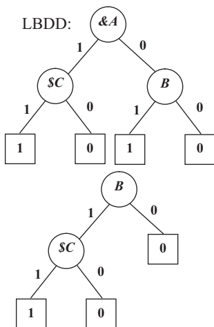
Fig. 8 The L-BDD for the fault tree shown in Fig. 2
