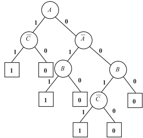
Fig. 7 ZBDD for the SFBDD shown in Fig. 3
