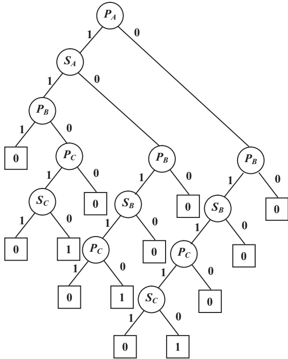
Fig. 6 Meta-products BDD for the SFBDD shown in Fig. 3
